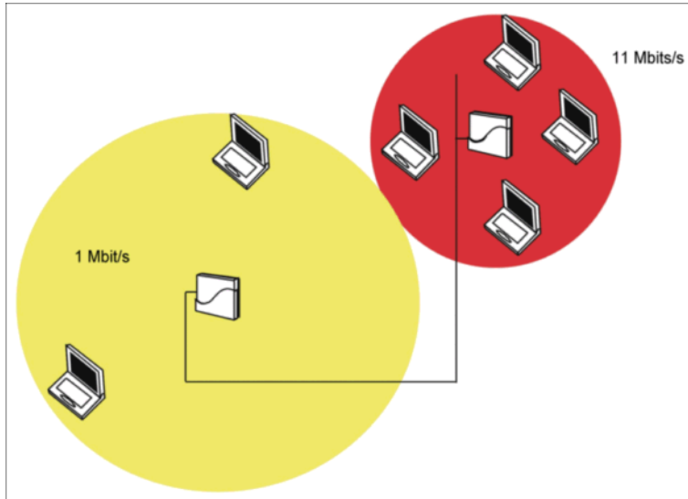
Figure 4-12 1 Mbit/s and 11 Mbit/s Multicast Rates
