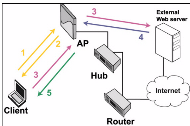
Figure 3-4 External Authentication
