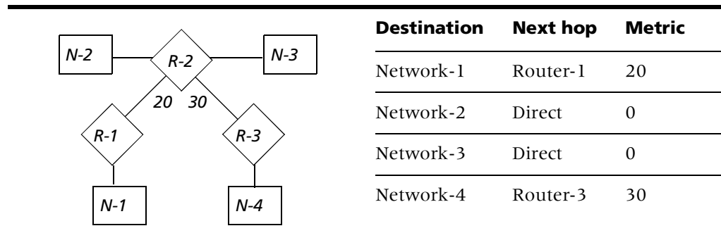
Figure 47. Shortest-path tree and resulting routing table for Router-2
