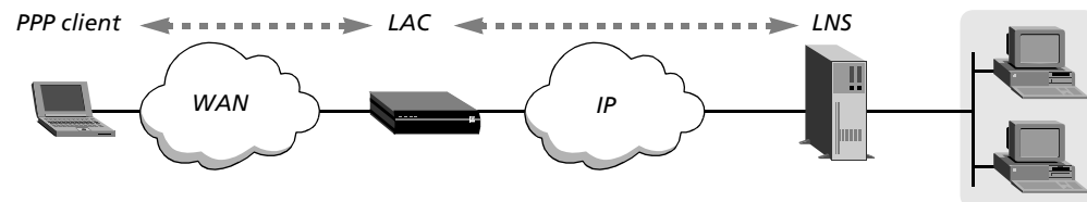
Figure 42. L2TP tunnel
