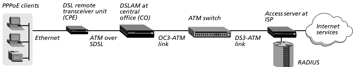
Figure 66. PPPoE configuration
