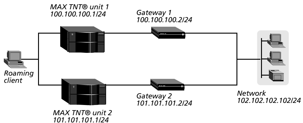
Figure 68. Using a pseudogateway
