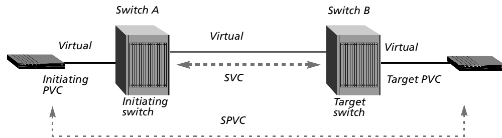
Figure 74. SPVC
