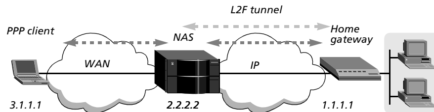
Figure 41. L2F tunneling
