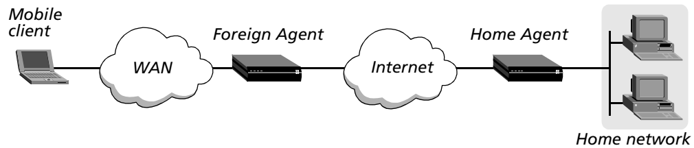
Figure 7. ATMP tunnel across the Internet
