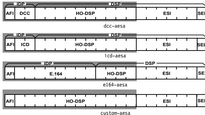
Figure 2. Subfields in the AESA address formats
