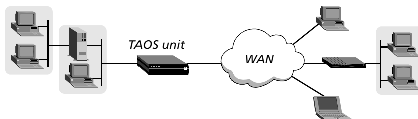
Figure 39. IPX-routing configuration
