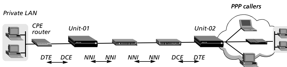
Figure 30. Frame relay network
