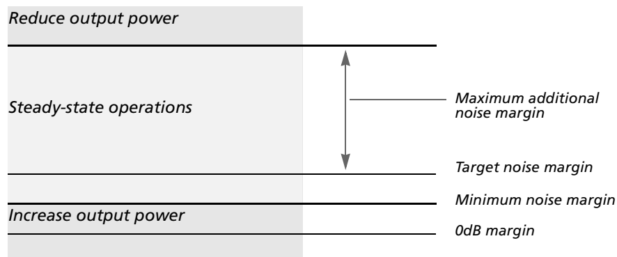
Figure 61. Noise margins
