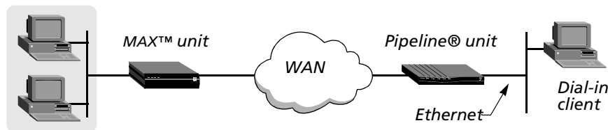
Figure 65. PPP connection
