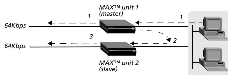
Figure 72. Packet flow from the Ethernet network
