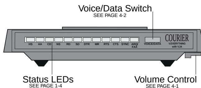
Figure 1-1. The Courier V.Everything Modem (Front).
