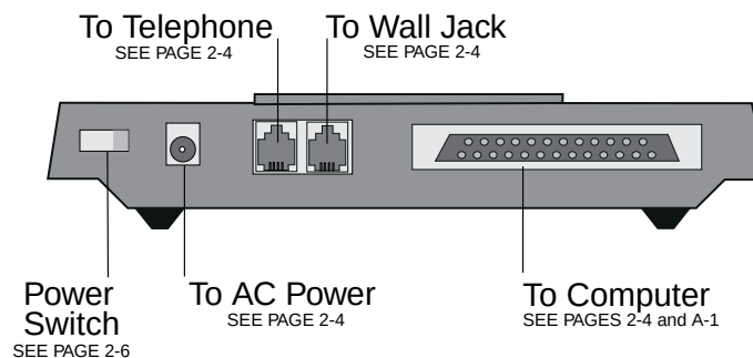
Figure 1-2. The Courier V.Everything Modem (Back).
