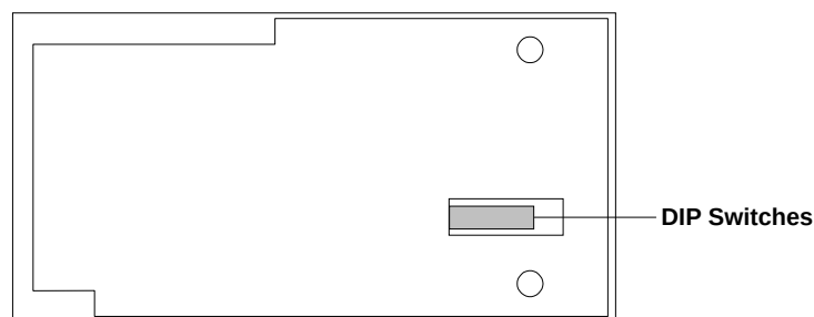
Figure 2-3. Location of the DIP Switches.
