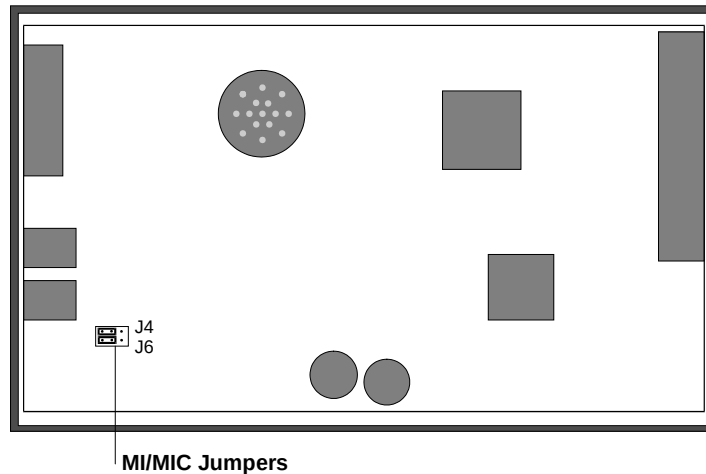
Figure 4-1. Location of the MI/MIC Jumpers.
