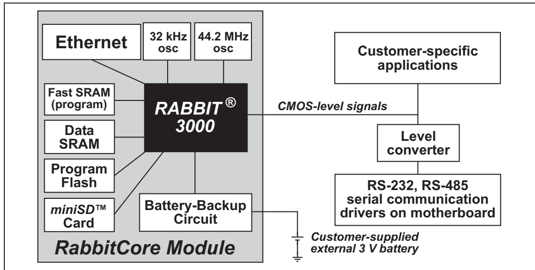
Figure 4. RCM3900 Subsystems
