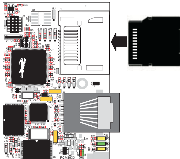
Figure 10. Insertion/Removal of miniSD Card
