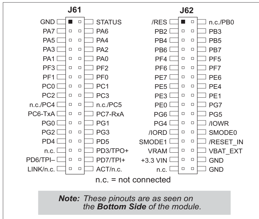
Figure 5. RCM3900 Pinouts
