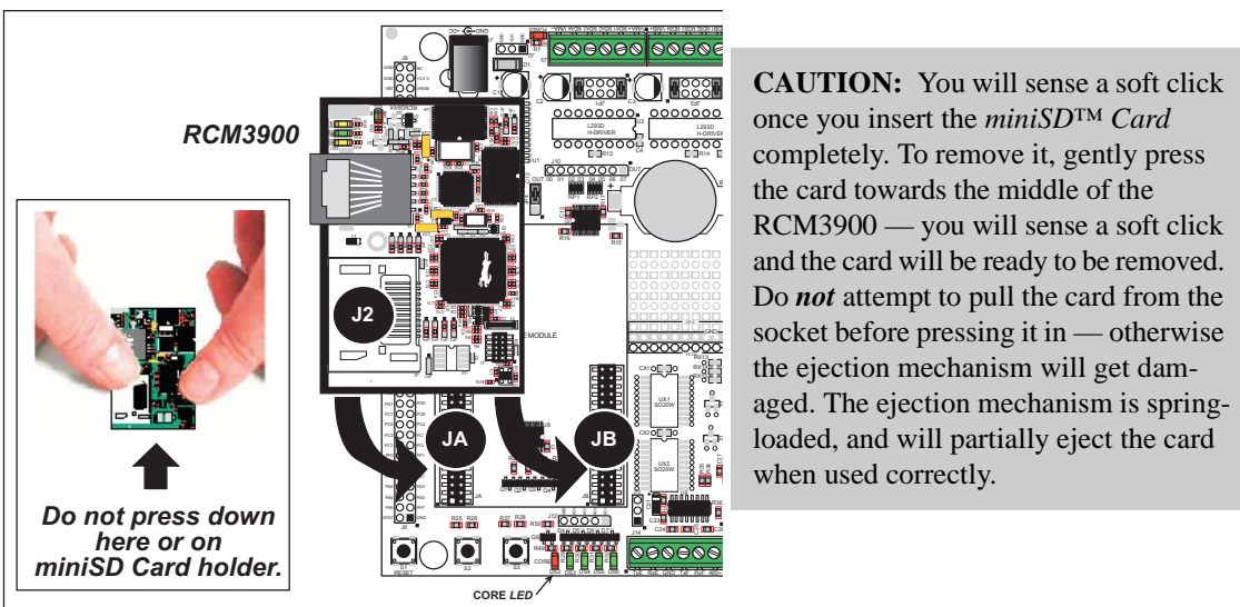
Figure 2. Install the RCM3900 Series on the Prototyping Board
