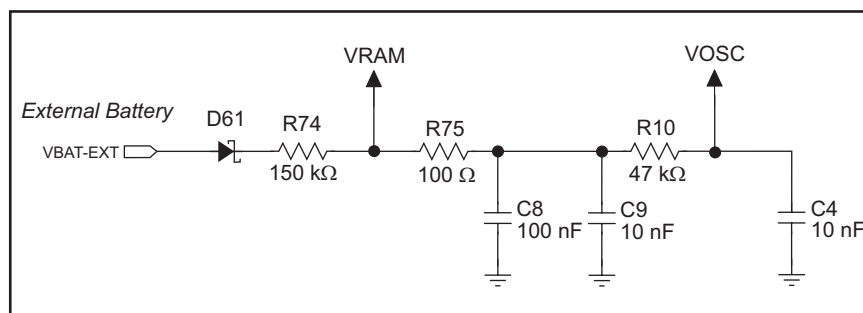
Figure D-2. RCM3900 Backup Battery Circuit
