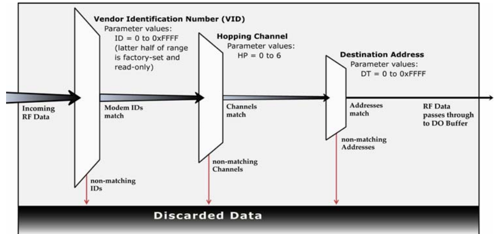
Figure 3.6. Filtration Layers Contained in the Header
