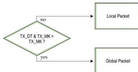
Figure 5-03. Address Recognition (@ the Transmitting RF Modem)
