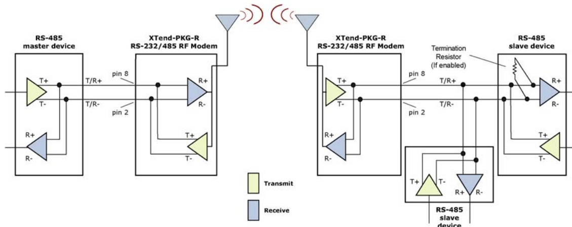
Figure 2-09. Figure 2-09. XTend RF Modem in an RS-485 (2-wire) half-duplex environment
