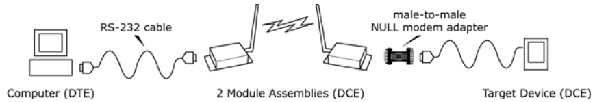
Figure B-04. Example of a MaxStream Radio Modem (DCE Device) connecting to another DCE device
