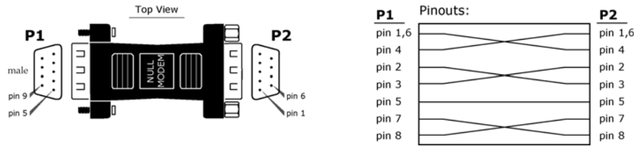
Figure B-04. Example of a MaxStream Radio Modem (DCE Device) connecting to another DCE device
