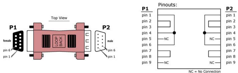
Figure B-06. Serial loopback adapter and pinouts
