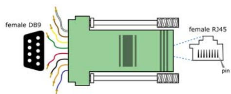
Figure 2-16. Female DB-9 to RJ-45 Adapter (green)
