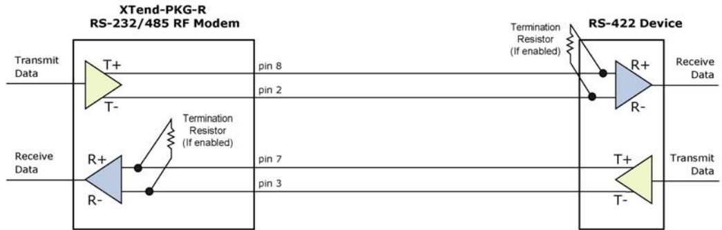
Figure 2-14. XTend RF Modem in an RS-422 environment
